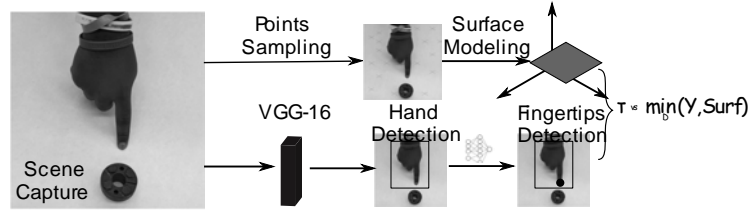
Figure 2. The framework of touch detection.
