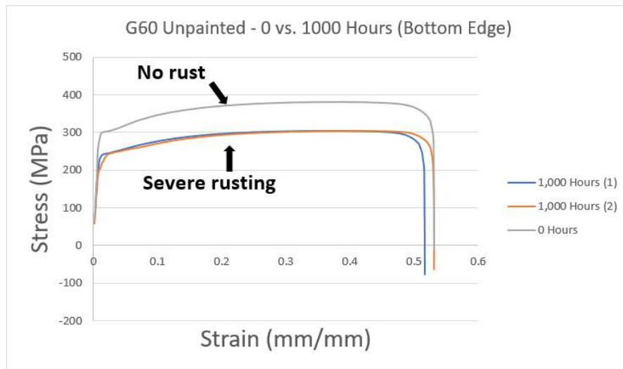
Figure 6: Stress-strain curve for the G60 unpainted samples with severe corrosion effects under the salt spray tests
