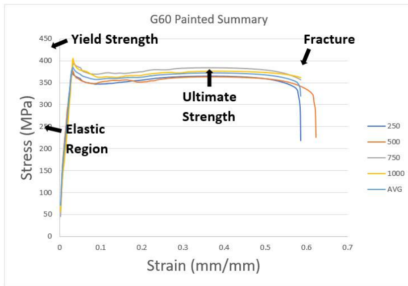
Figure 1: Stress-strain curve of the G60 powder-coated metal sheet samples as a function of salt spray exposure times
