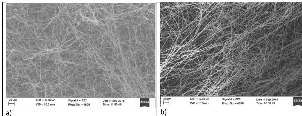
Figure 1: the SEM images of the same nanofiber membranes a) without and b) with heat treatment processes.
