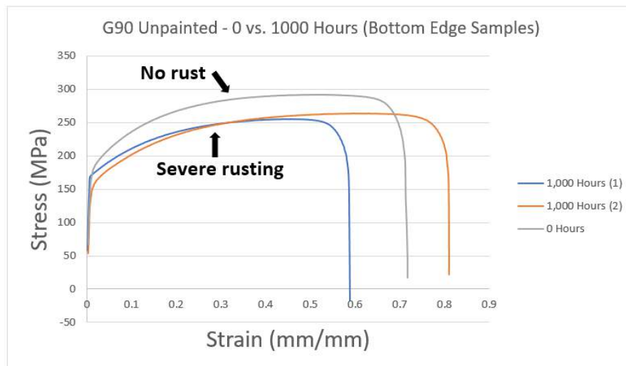
Figure 7: Stress-strain curve for G90 unpainted samples with severe corrosion effects
