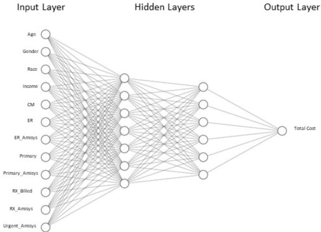
Figure 3: Visual Representation of a 7, 6 NN
