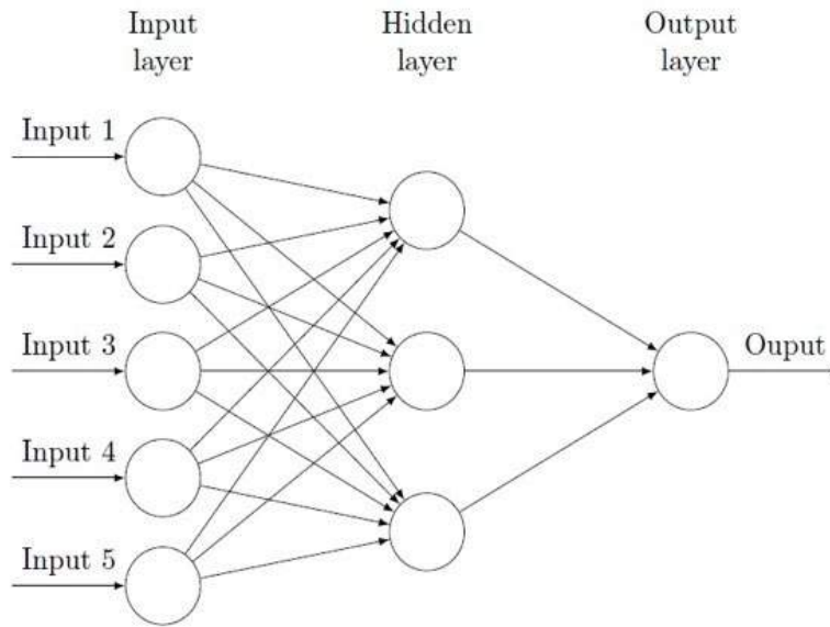
Figure 1: Neural Network with one input layer of 5 and one hidden layer of 3
