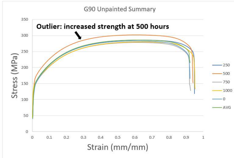
Figure 5: Stress-strain curve for the G90 unpainted samples as a function of exposure times
