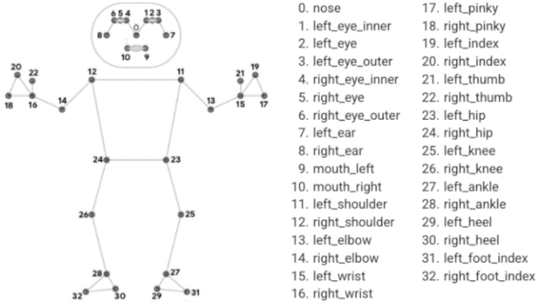
Figure 2. MediaPipe keypoints representation of a human body (MediaPipe, 2021)
