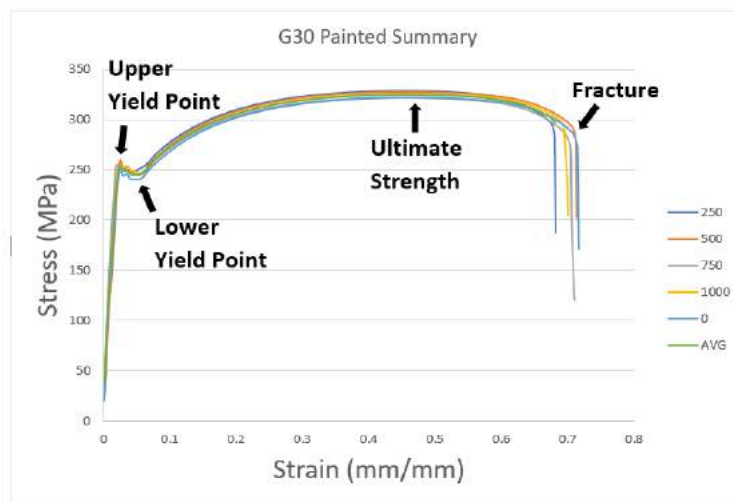
Figure 3: Stress-strain curve for G30 pre-painted samples as a function of the salt spray exposure times
