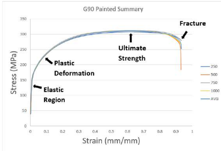
Figure 2: Stress-strain curve for the G90 powder-coated sheet samples as a function of salt spray exposure time
