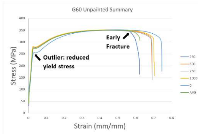
Figure 4: Stress-strain curve for the G60 unpainted samples as a function of exposure times
