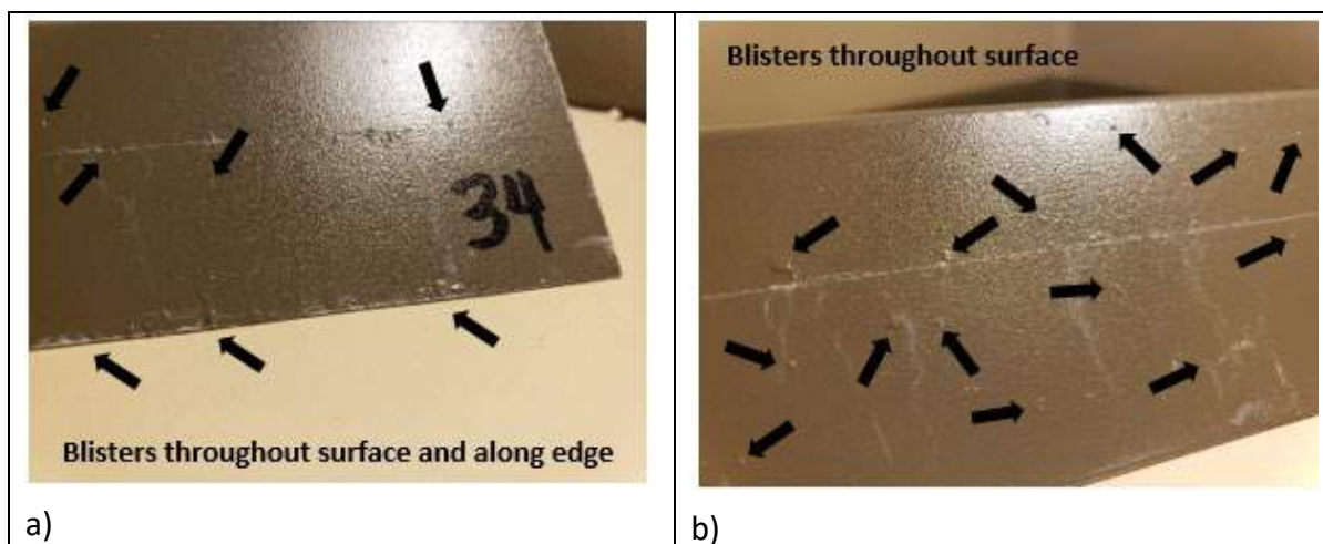
Figure 8: Blistering effects on the G30 samples for a) 750 hours and b) 1,000 hours
