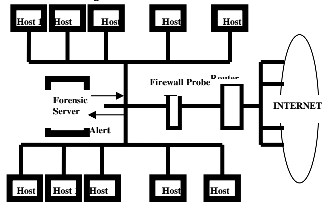
Fig.1 Logical Architecture for the Forensic Profiling System. The forensic clients are composed of hosts, servers, firewalls and the router in the network.
