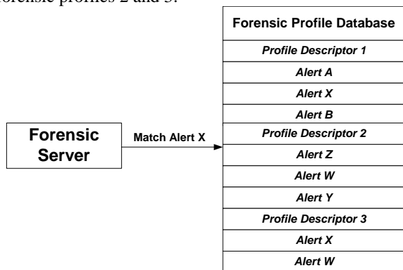
Fig. 2 The forensic server scans for Alert X in the forensic profile database. The scan results in transforming Profile Descriptors 1 and 3 as active.
