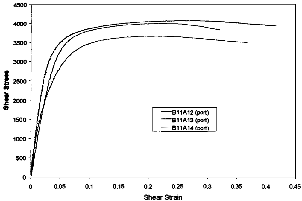
FIGURE F-5. PTM&W ES6292 ADHESIVE SHEAR STRESS-STRAIN CHART FOR T \approx 0.013 in. RTD
