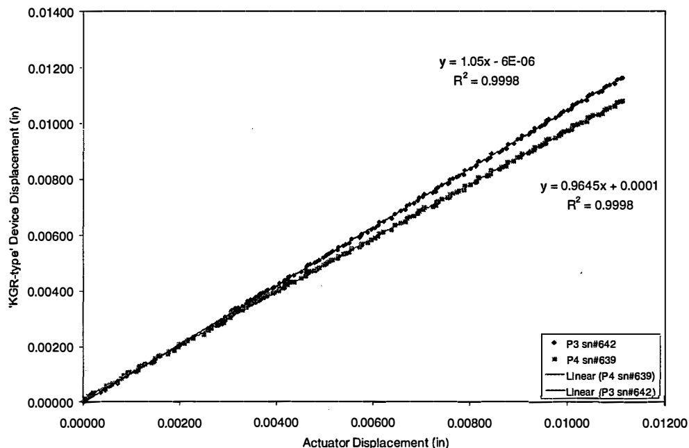
FIGURE A-1. EXAMPLE OF CALIBRATION CURVES FOR THE KGR-TYPE DEVICES CALIBRATION FACTOR (Note that actual displacement and the measured displacement from the devices are not a 1:1 correlation.)
