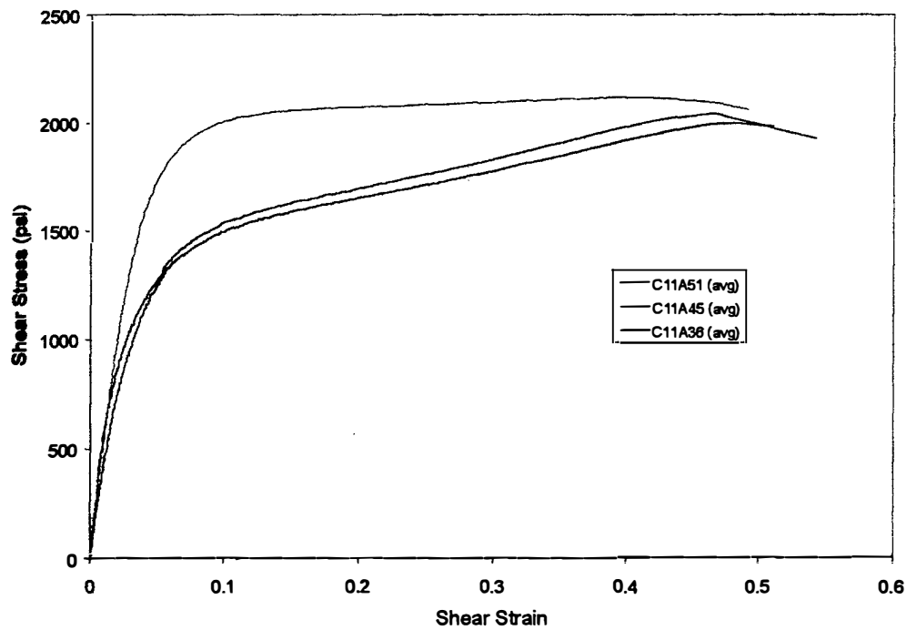
FIGURE F-17. MGS A100/B100 ADHESIVE SHEAR STRESS-STRAIN CHART FOR T \approx 0.013 in. ETD 200°F
