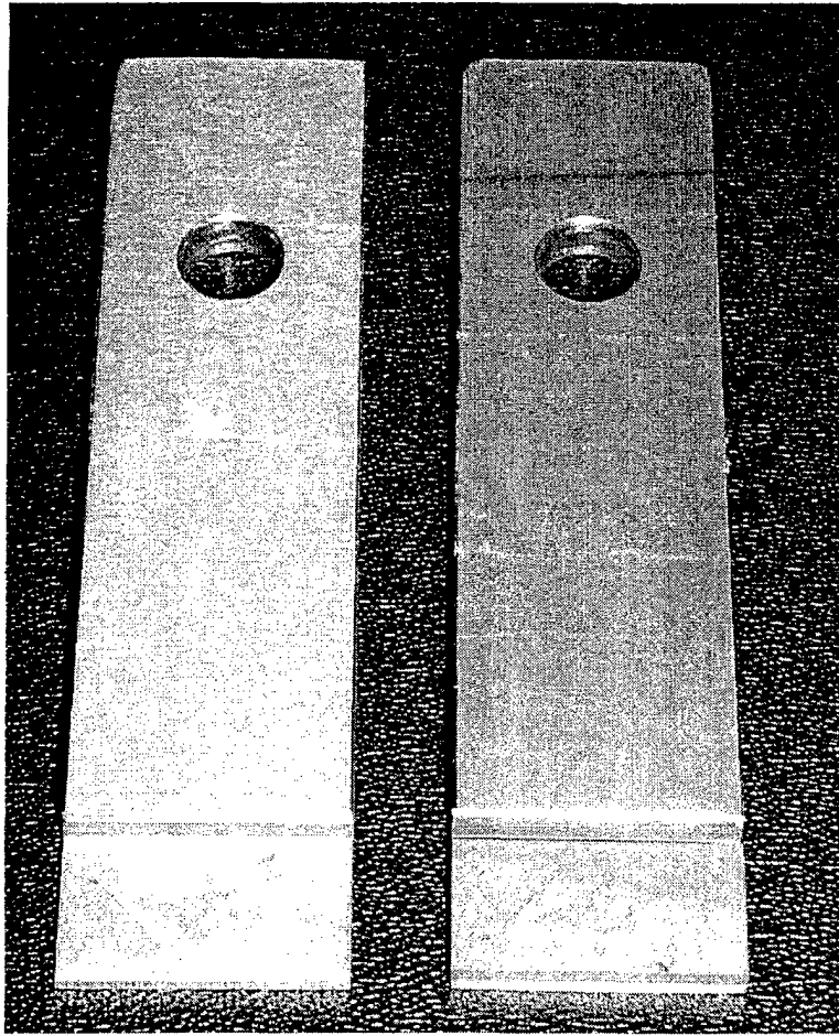
FIGURE 36. EXAMPLE OF COHESIVE/ADHESIVE FAILURE OF ALUMINUM ADHEREND ASTM D 3165 SPECIMEN. NOTE THE <50% ADHESIVE FAILURE ON THE UPPER PORTION OF THE RIGHT HALF OF SPECIMEN.
