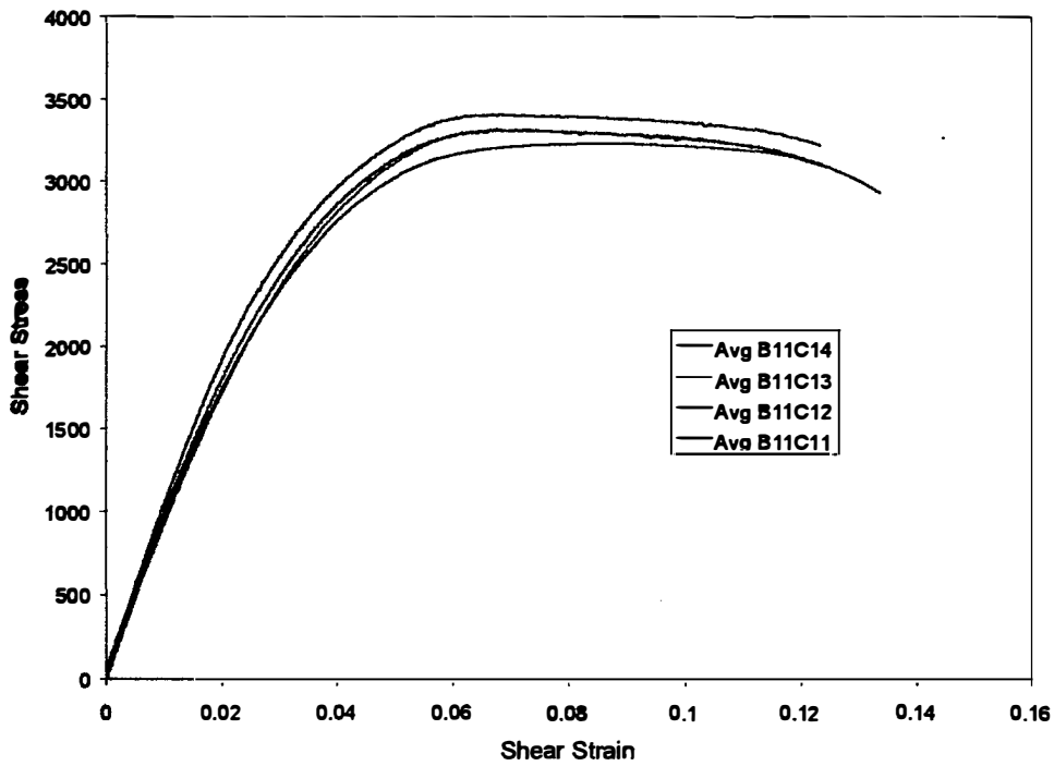
FIGURE F-7. PTM&W ES6292 ADHESIVE SHEAR STRESS-STRAIN CHART FOR T \approx 0.082 in. RTD
