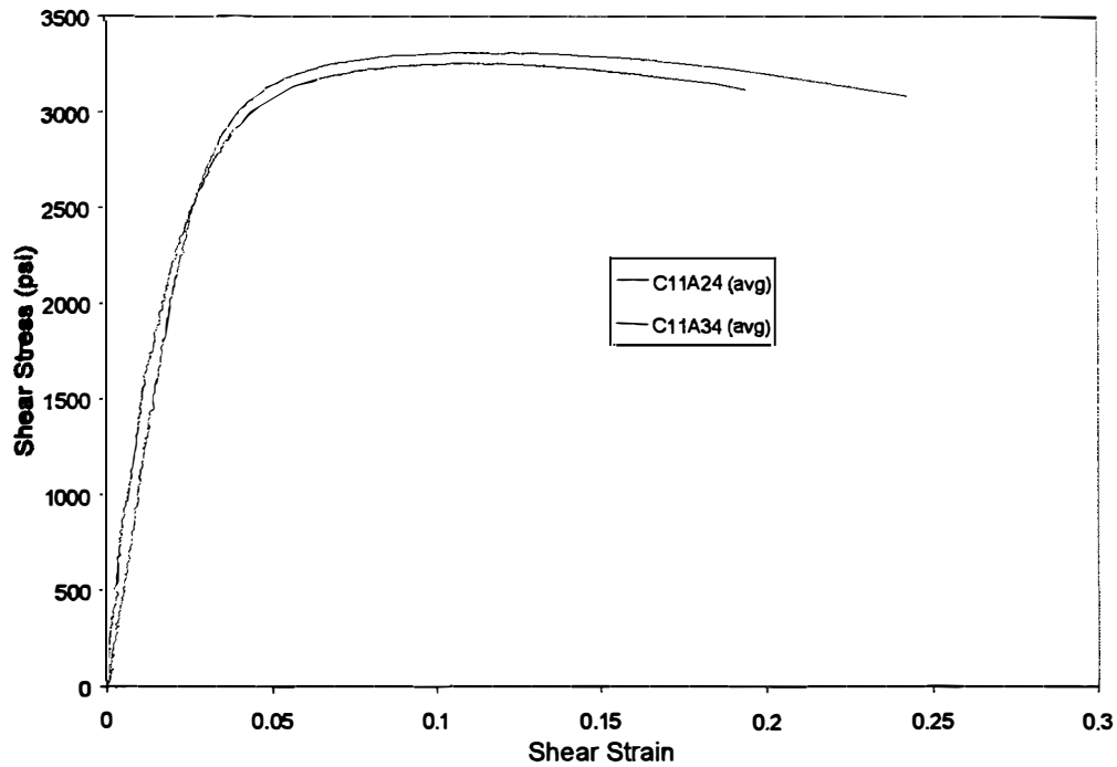
FIGURE F-15. MGS A100/B100 ADHESIVE SHEAR STRESS-STRAIN CHART FOR T \approx 0.013 in. ETD 160°F
