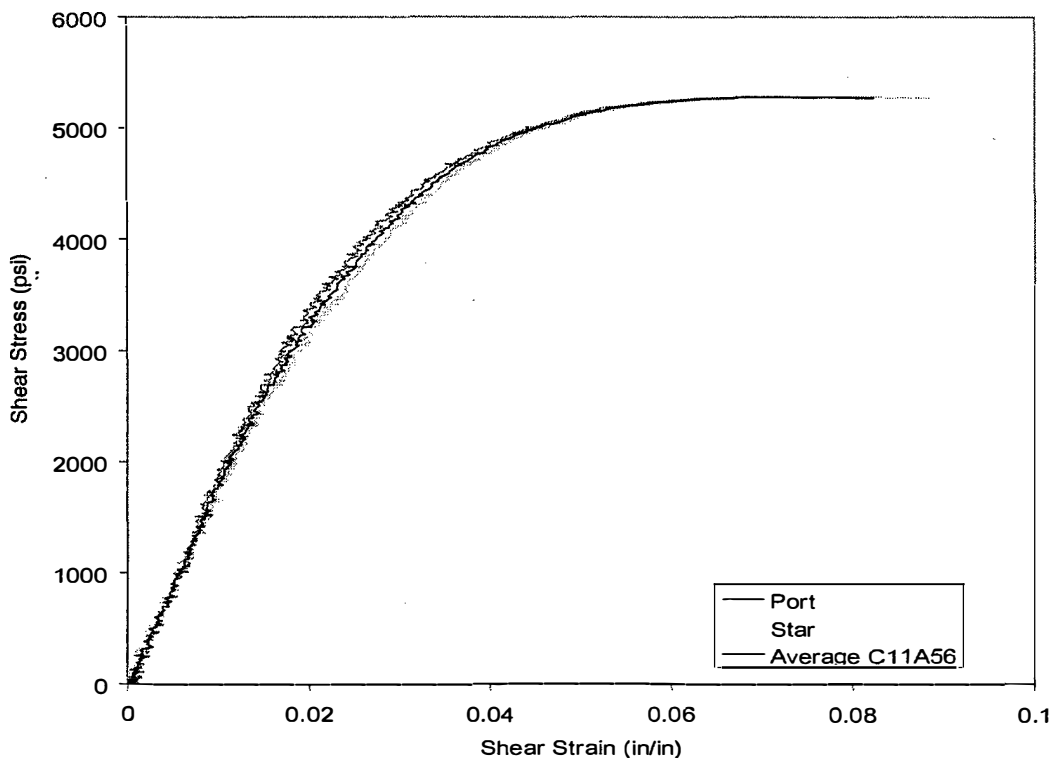
FIGURE 13. EXAMPLE OF AN ADHESIVE SHEAR STRESS-STRAIN CHART (This chart shows the readings from both KGR-type devices and the average reading (MGS adhesive, t = 0.013'' , RTD test))
