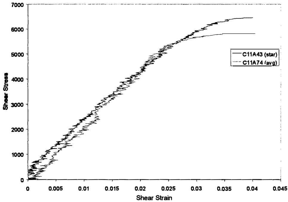
FIGURE F-13. MGS A100/B100 ADHESIVE SHEAR STRESS-STRAIN CHART FOR T \approx 0.013 in. CD
