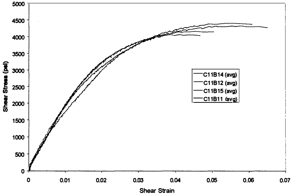
FIGURE F-10. MGS A100/B100 ADHESIVE SHEAR STRESS-STRAIN CHART FOR T \approx 0.042 in. RTD
