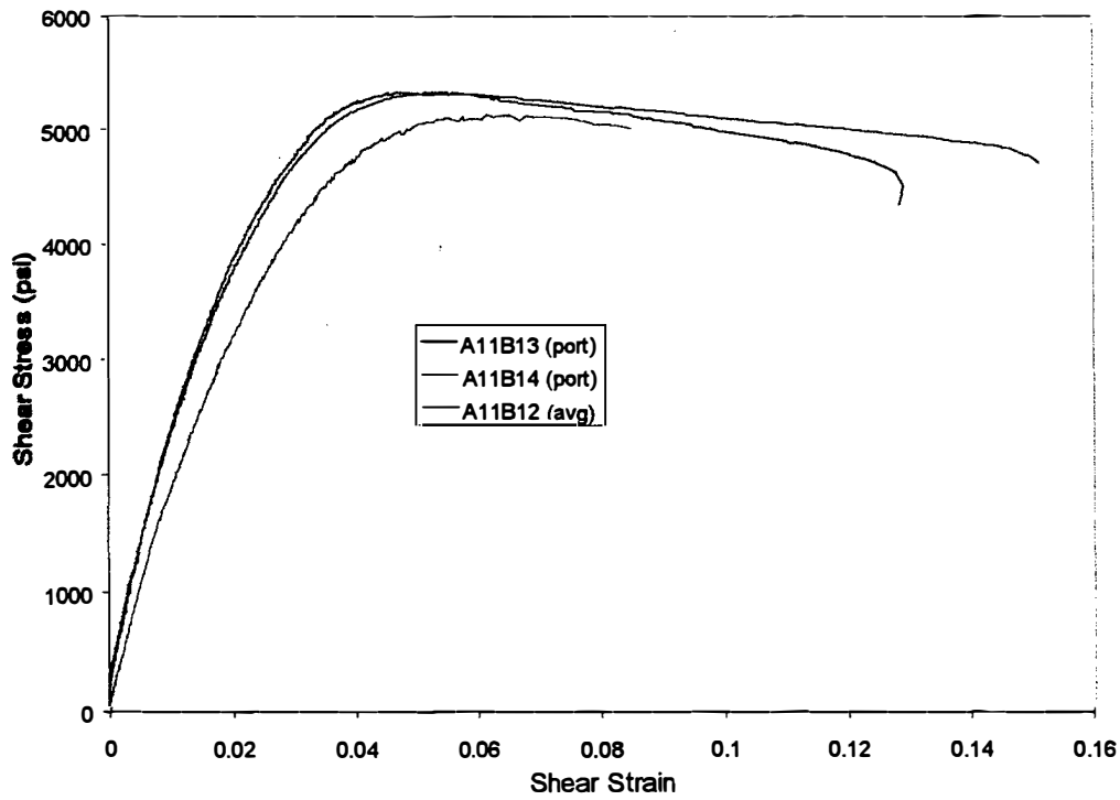
FIGURE F-2. HYSOL EA9394 ADHESIVE SHEAR STRESS-STRAIN CHART FOR T \approx 0.060 in. RTD
