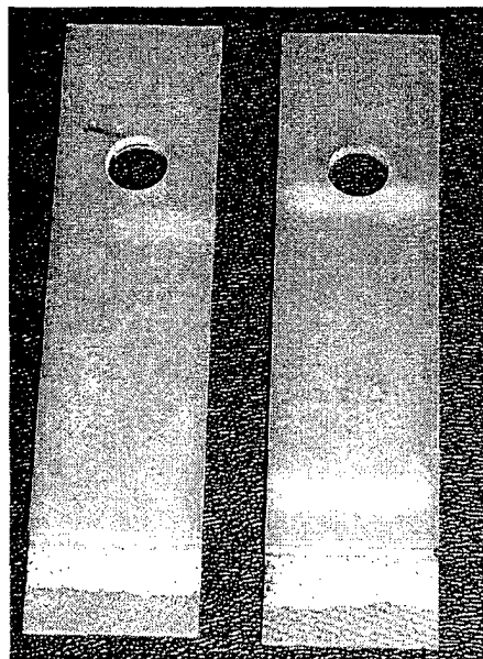
FIGURE 35. EXAMPLE OF FIRST-PLY FAILURE IN FIBERGLASS/EPOXY ASTM D 3165 SPECIMEN. THE FIRST-PLY OF LAMINATE CAN BE SEEN STILL ADHERING TO THE ADHESIVE ON BOTH PORTIONS OF THE SPECIMEN.
