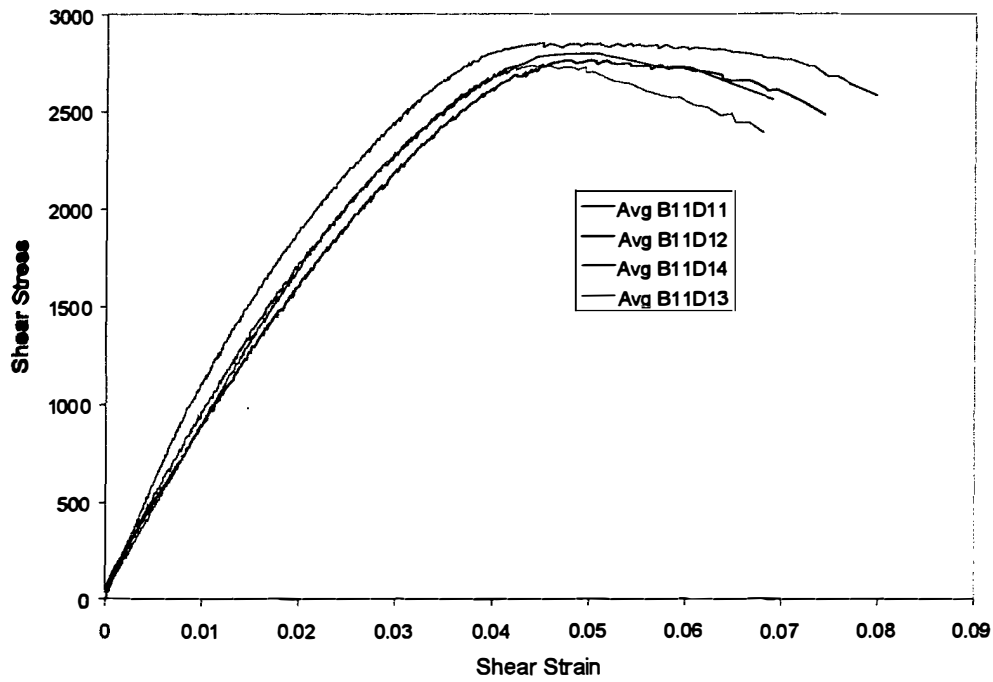
FIGURE F-8. PTM&W ES6292 ADHESIVE SHEAR STRESS-STRAIN CHART FOR T \approx 0.120 in. RTD
