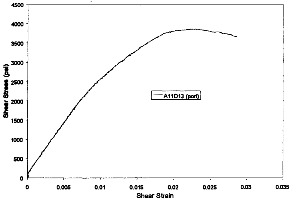
FIGURE F-4. HYSOL EA9394 ADHESIVE SHEAR STRESS-STRAIN CHART FOR T \approx 0.135 in. RTD
