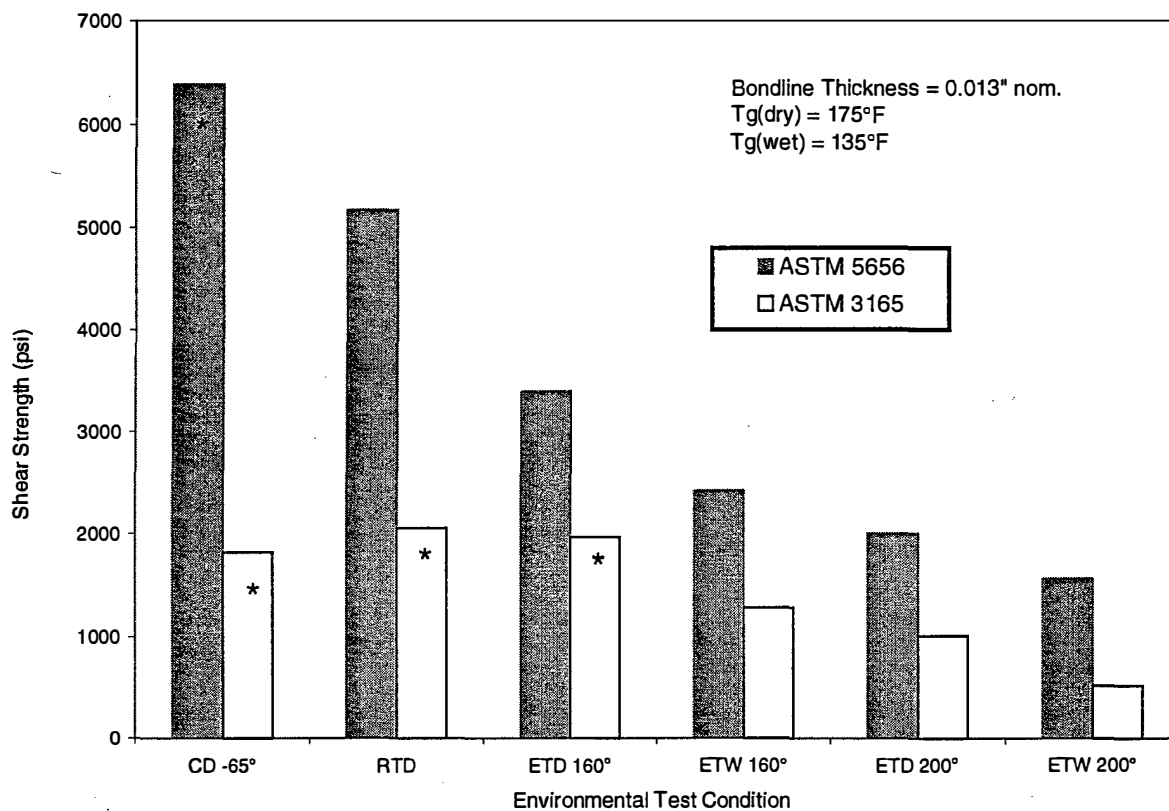
FIGURE 44. APPARENT SHEAR STRENGTH OF MGS ADHESIVE VERSUS ENVIRONMENTAL CONDITION FOR ALUMINUM THICK-ADHEREND SPECIMENS AND C/Ep THIN-ADHEREND SINGLE-LAP SHEAR SPECIMENS (Starred data denotes noncohesive failures)
