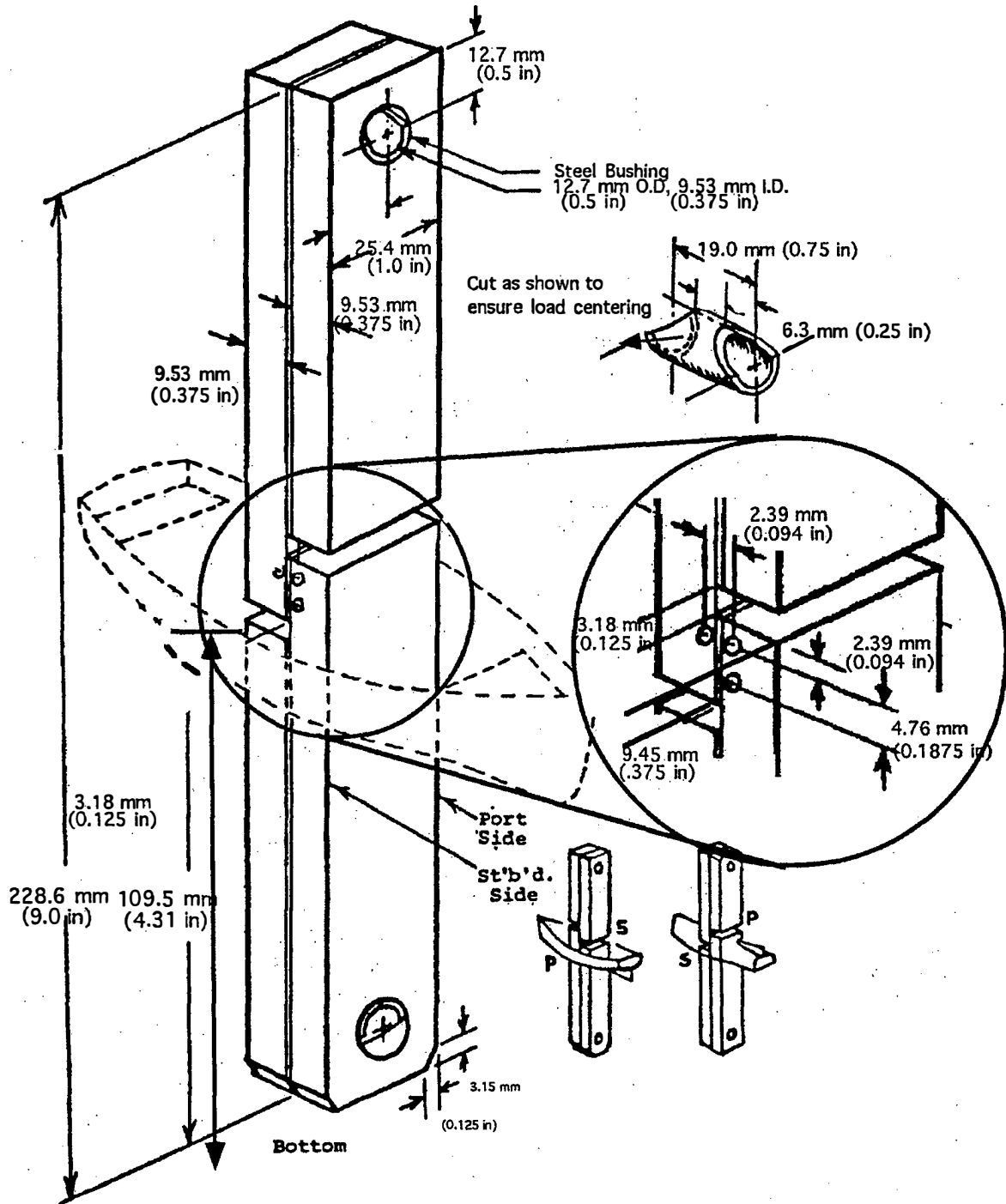
FIGURE 6. ASTM D 5656 SPECIFICATIONS FOR SPECIMEN DIMENSIONS
