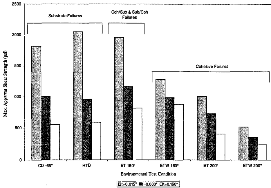
FIGURE 40. AVERAGE MAXIMUM APPARENT SHEAR STRENGTH VERSUS ENVIRONMENTAL CONDITION FOR THREE DIFFERENT BONDLINE THICKNESSES (ASTM D 3165, C/Ep adherends, MGS adhesive)
