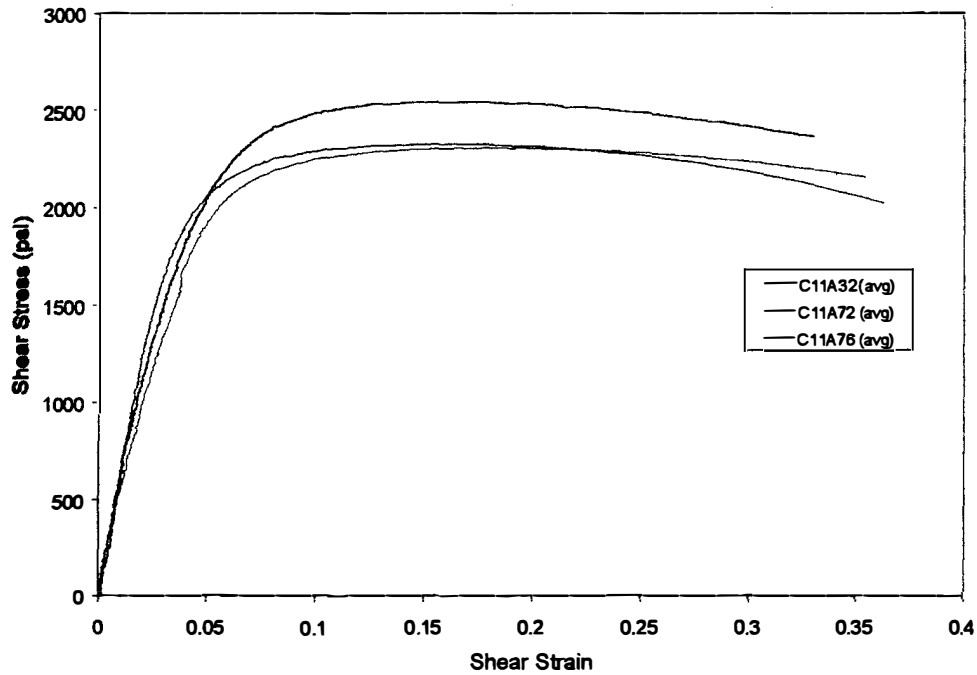
FIGURE F-16. MGS A100/B100 ADHESIVE SHEAR STRESS-STRAIN CHART FOR T \approx 0.013 in. ETW 160°F
