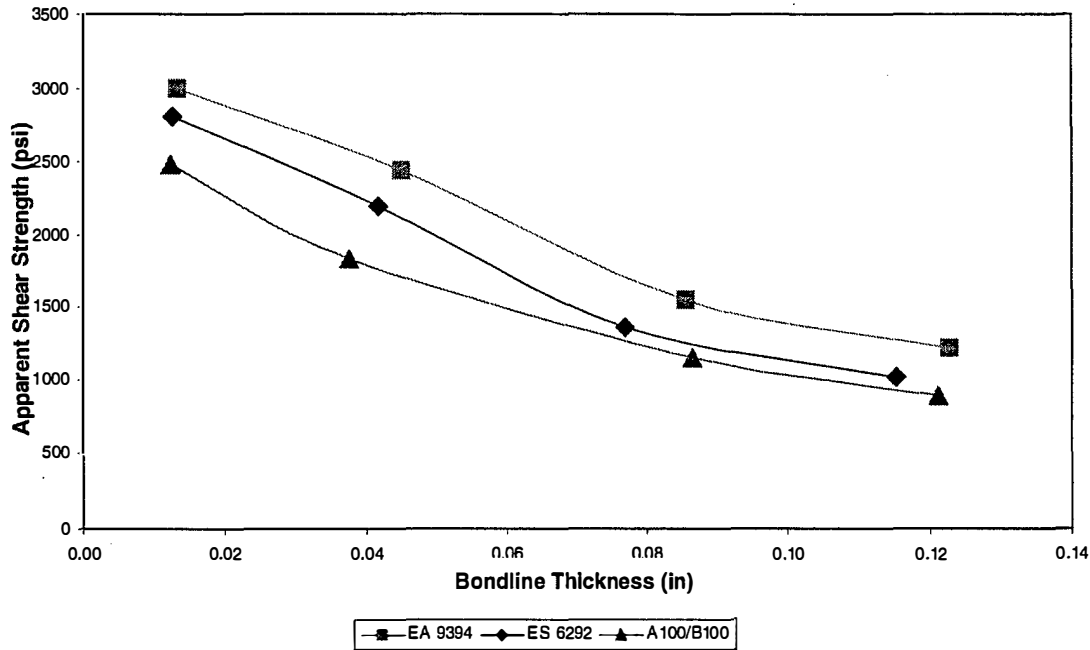
FIGURE 32. APPARENT SHEAR STRENGTH OF ALL THREE ADHESIVES VERSUS BONDLINE THICKNESS WITH ALUMINUM ADHERENDS (ASTM D 3165) (Failure modes are shown in table 24)
