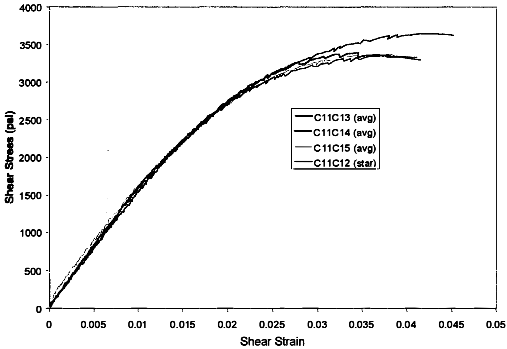
FIGURE F-11. MGS A100/B100 ADHESIVE SHEAR STRESS-STRAIN CHART FOR T \approx 0.082 in. RTD
