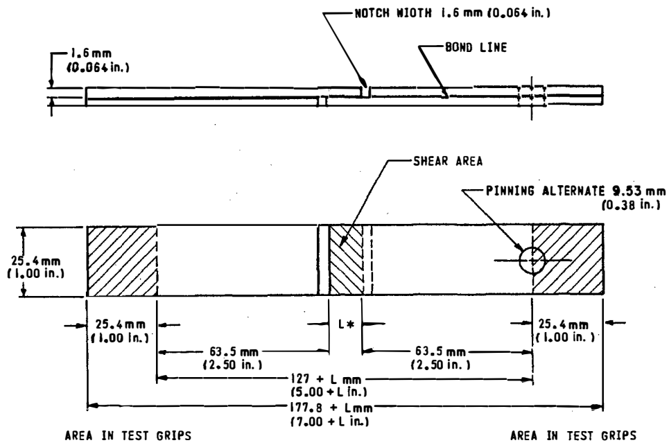
FIGURE 2. ASTM D 3165 TEST SPECIMEN PROFILE [6]
