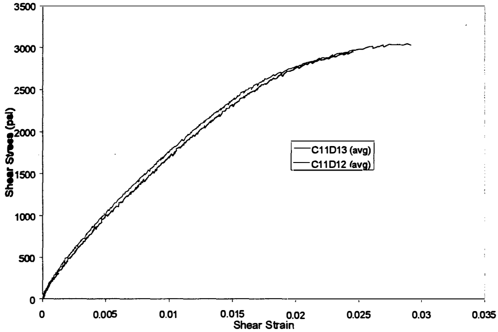
FIGURE F-12. MGS A100/B100 ADHESIVE SHEAR STRESS-STRAIN CHART FOR T \approx 0.120 in. RTD
