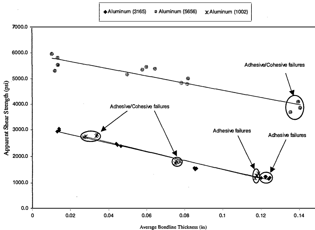
FIGURE 37. COMPARISON OF ASTM D 1002 AND D 3165 APPARENT SHEAR STRENGTH VERSUS BONDLINE THICKNESS (Hysol 9394 adhesive)
