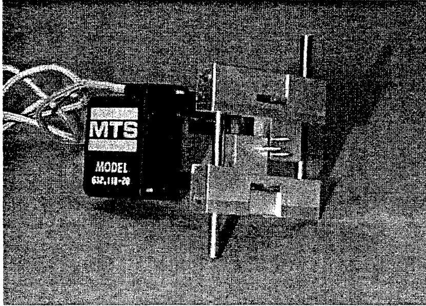
FIGURE 7. THE ORIGINAL KGR-TYPE EXTENSOMETER
