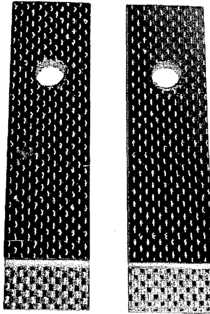
FIGURE 34. EXAMPLE OF FIRST-PLY FAILURE IN CARBON/EPOXY ASTM D 3165 SPECIMEN. THE RIGHT PORTION OF THE SPECIMEN SHOWS PART OF THE FIRST-PLY FROM HE LEFT PORTION STILL ADHERING TO ADHESIVE.
