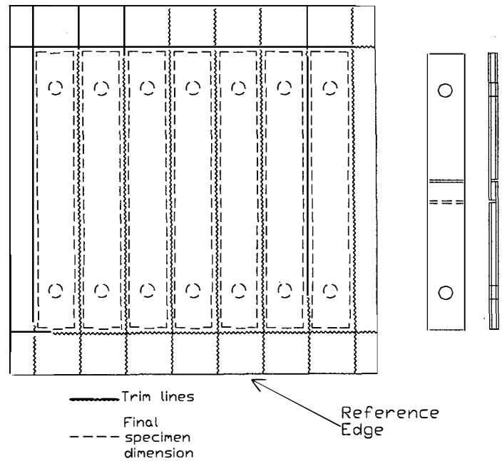
FIGURE 22. SCHEMATIC OF THE BONDED ALUMINUM ASTM D 3165 SUBPANEL
