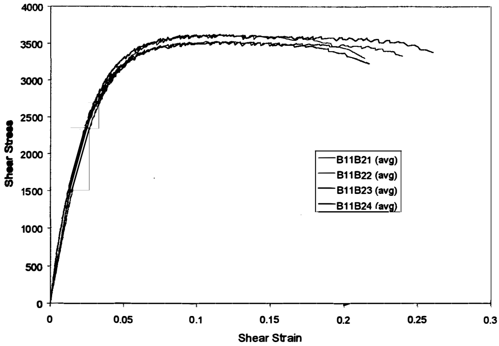
FIGURE F-6. PTM&W ES6292 ADHESIVE SHEAR STRESS-STRAIN CHART FOR T \approx 0.042 in. RTD
