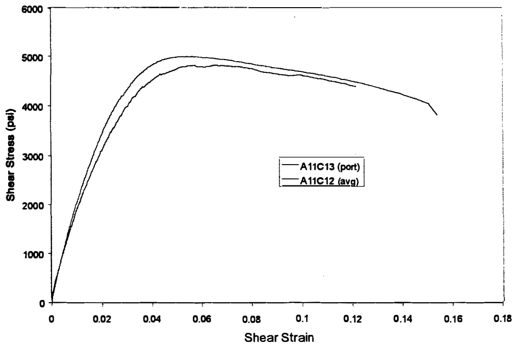
FIGURE F-3. HYSOL EA9394 ADHESIVE SHEAR STRESS-STRAIN CHART FOR T \approx 0.080 in. RTD
