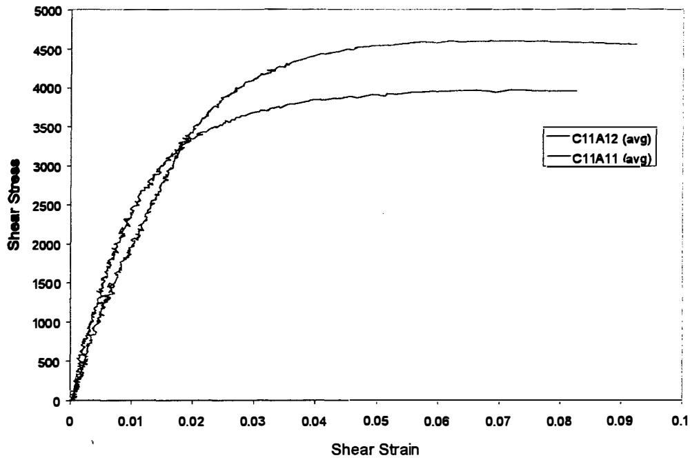
FIGURE F-9. MGS A100/B100 ADHESIVE SHEAR STRESS-STRAIN CHART FOR T \approx 0.013 in. RTD
