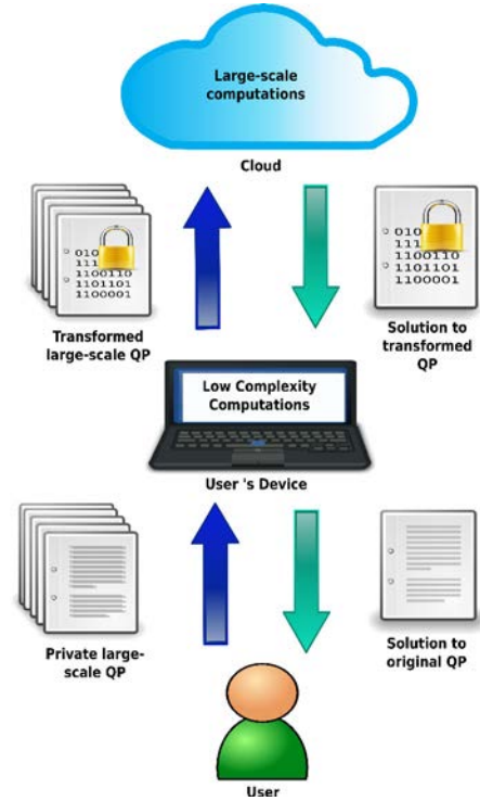
Figure 1: An Architecture for Securely Outsourcing QPs.
