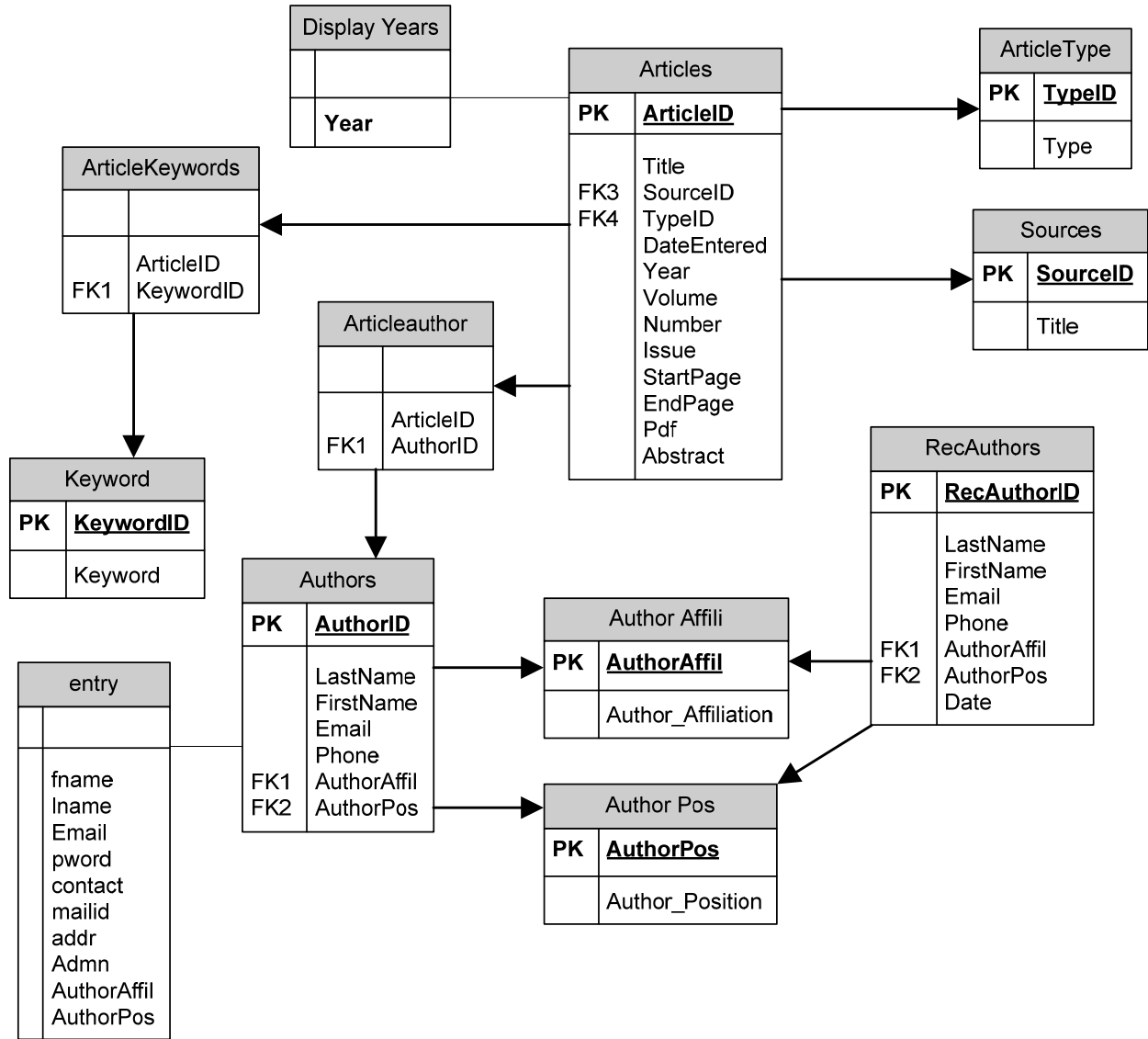
FIGURE 4 THE SOFTWARE PROTOTYPE DATABASE
